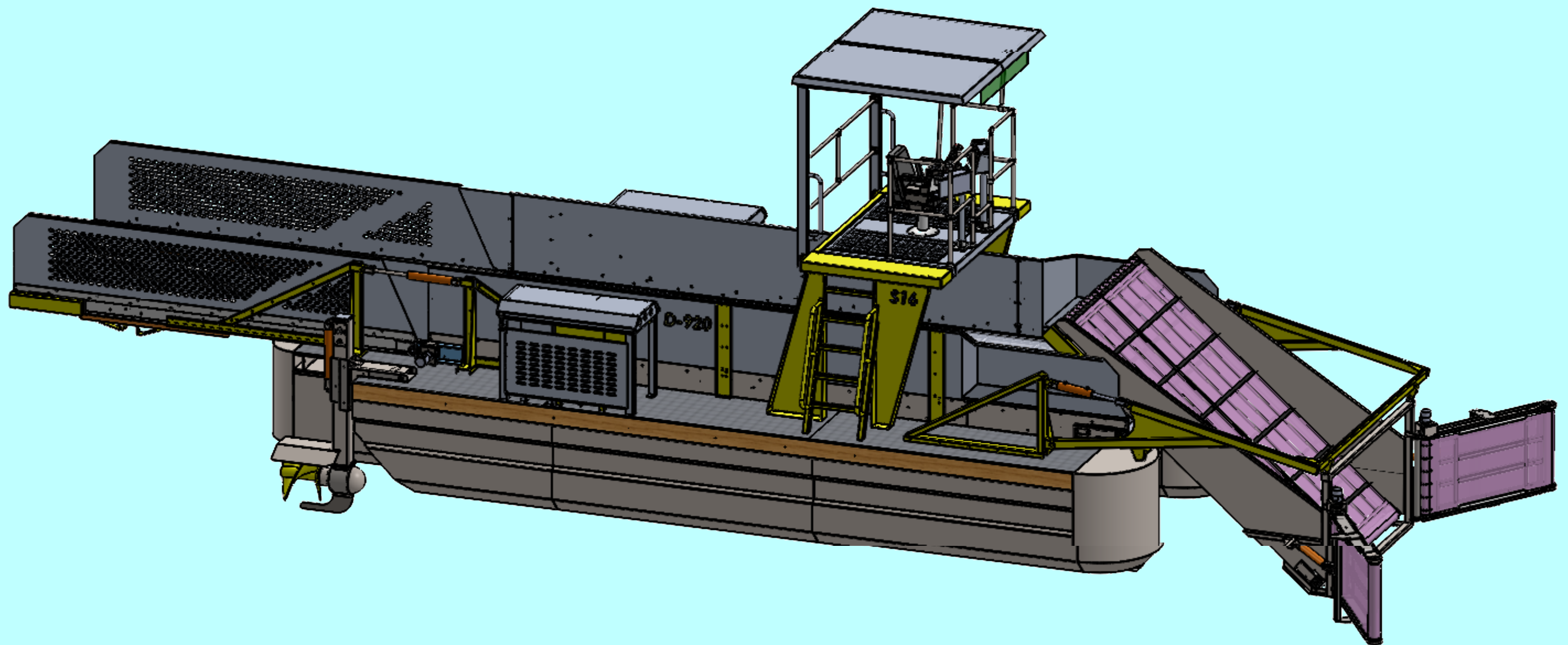
Series F-920 , Model S16 • Collecting swath width: 16' / 4.88 m • Cargo: 1000 ft 3 /28 m 3 Power: 114 HP / 85 kW • Length: 48.5' / 14,80 m • Width: 11.92' / 3,64 m • Weight: 19500 lbs./8700 kg
