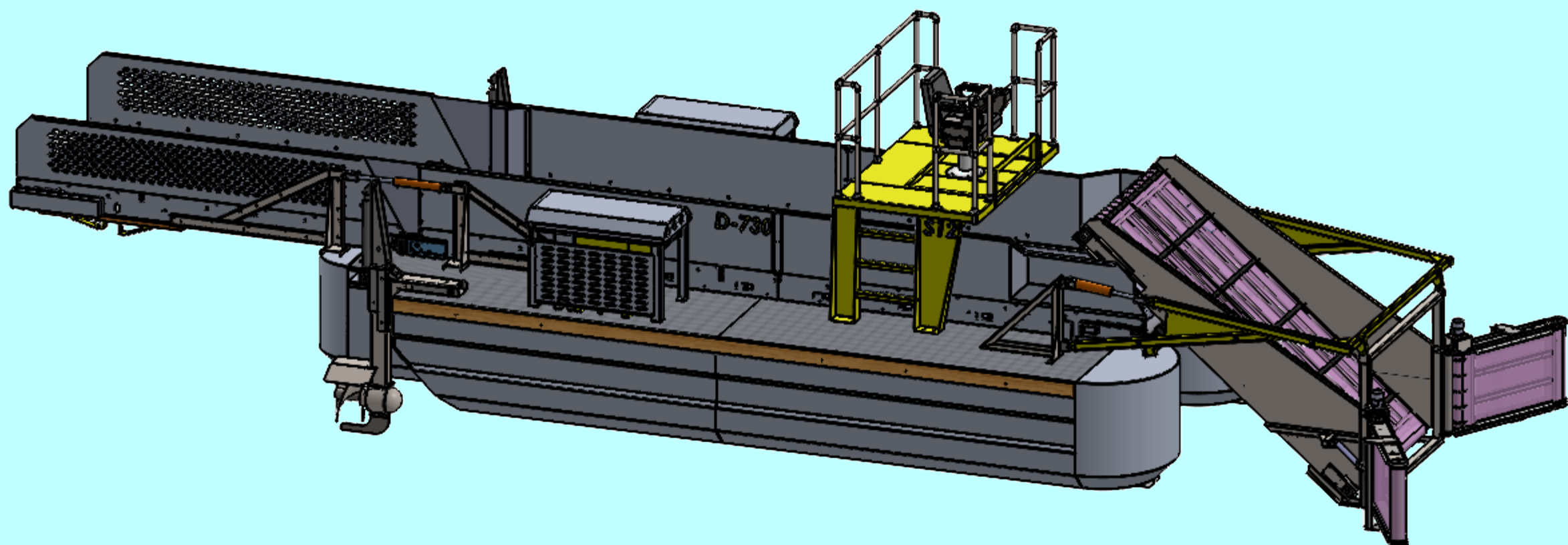
Series F-730 , Model S12 • Collecting swath width: 12' / 3,65 m • Cargo: 500 ft 3 / 14 m 3 Power: 75 HP / 56 kW • Length: 41' / 12,50 m • Width: 10.92' / 3,28 m • Weight: 12000 lbs./5400 kg
