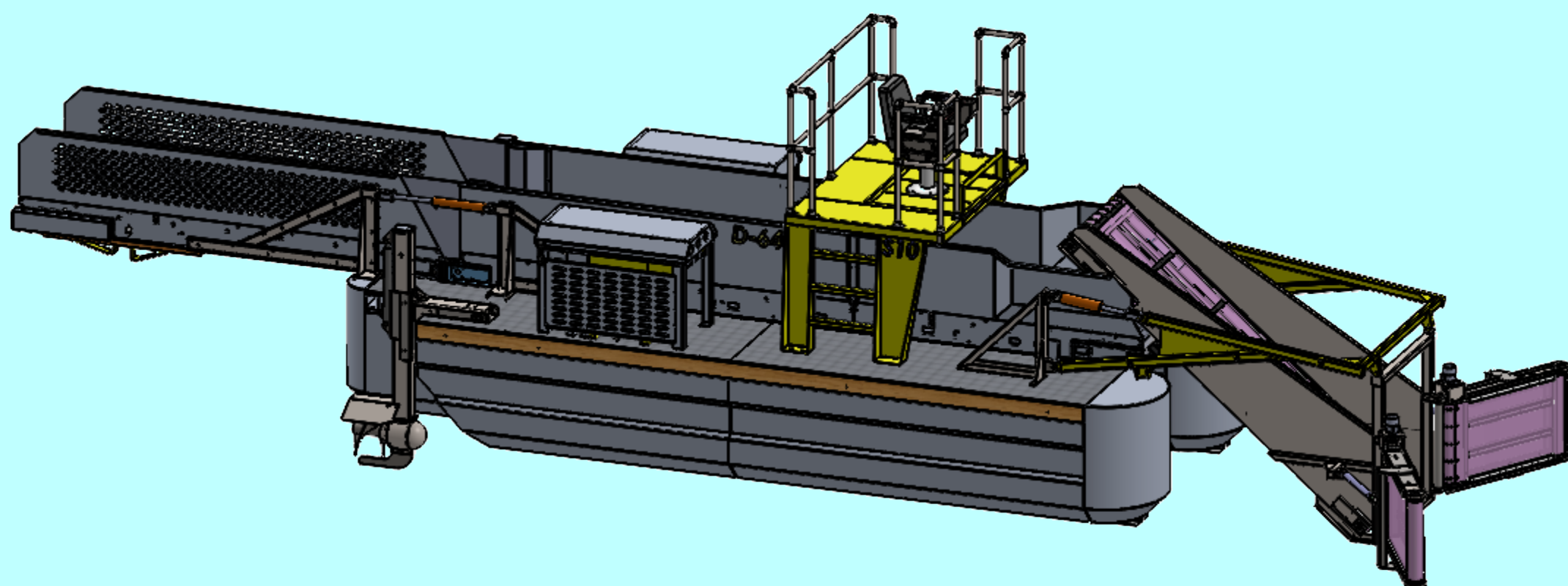
Series F-640 , Model S10 • Collecting swath width: 10' / 3,05 m • Cargo: 250 ft 3 /7m 3 Power: 50HP / 37kW • Length: 38' / 11.60 m • Width: 8.5' / 2.60 m • Weight: 8000 lbs./3600 kg
